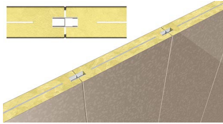
Type 2SM wall panel construction.
