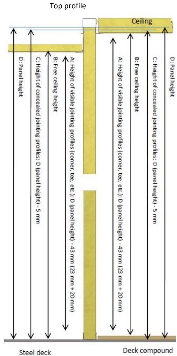
Heights of components
